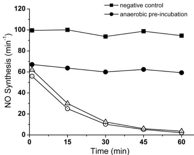
Fig. 2. Time and oxygen dependence of iNOS inhibition by BYK191023. Murine iNOS ( 2.5 \text{ } \mu\text{M} ) was preincubated for the indicated time with 10 \text{ } \mu\text{M} BYK191023 and 1 \text{ mM} NADPH at room temperature as described under Materials and Methods . Rates of NO synthesis were determined using the oxyhemoglobin assay. Empty circles ( \circ ) and triangles ( \Delta ) indicate, respectively, that superoxide dismutase and catalase were absent or present in the preincubation mixture. Filled circles ( \bullet ) represent activity measurements during anaerobic preincubation of iNOS. The data are the mean of three independent experiments. Negative control ( \blacksquare ) indicates that iNOS was preincubated in the absence of inhibitor.
