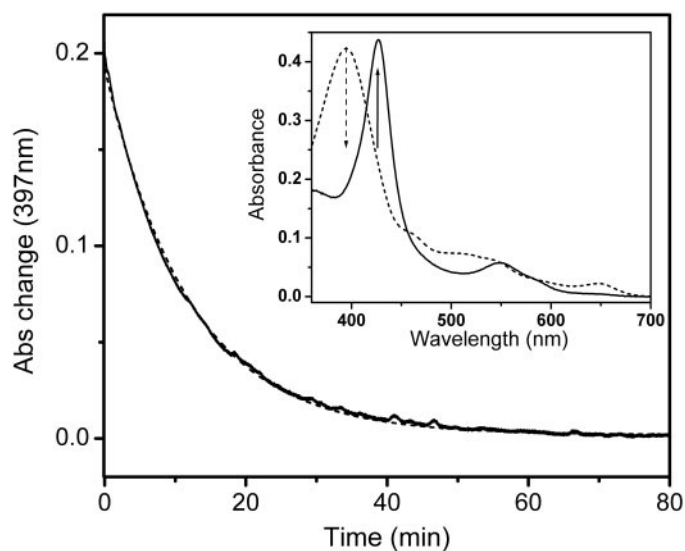
Fig. 4. Kinetics of BYK191023 dissociation. BYK191023 dissociation measured after the addition of 25 \text{ mM} imidazole was followed spectrally by monitoring the absorbance decrease at 397 \text{ nm} . The imidazole displaced BYK191023 completely in about 70 min. The curve was fitted using a first-order exponential decay equation to determine the apparent k_{\text{off}} . The inset shows the initial spectrum of BYK191023 bound iNOS (---) and 80 min after addition of 25 \text{ mM} imidazole (—). Imidazole binding to iNOS converts the heme iron from a high-spin state (Soret peak at 396 \text{ nm} ) to a low-spin state (Soret peak at 427 \text{ nm} ).
